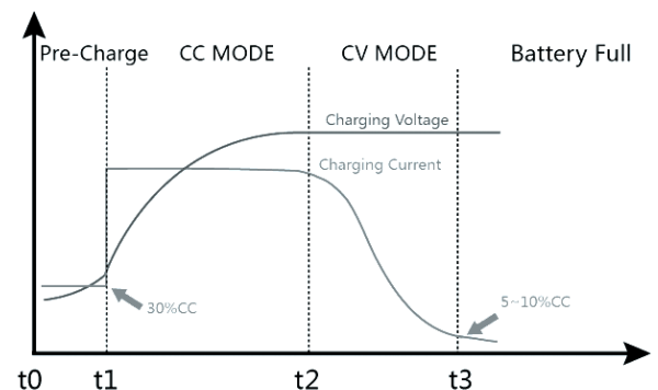
Figure 2. Charging characteristic curve.
